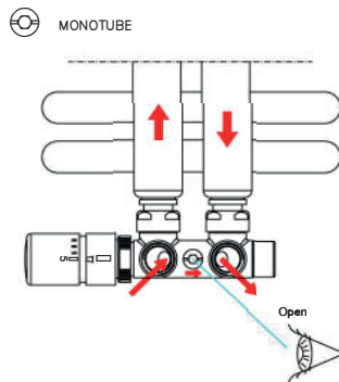
Angle version
