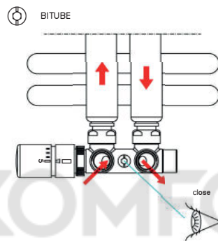
Angle version
