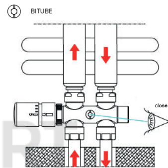
Straight version
