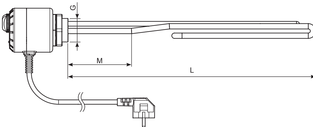
Fig. 8. ME 1030 heating module.
