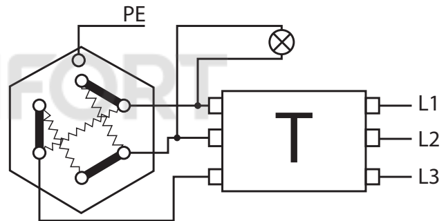
Fig. 5 Electrical diagram ME 2120 - ME 2180.
