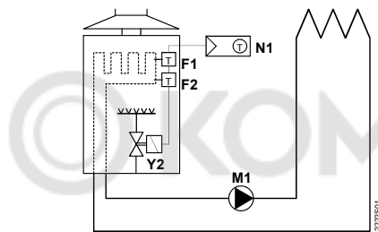
Room temperature controller with direct control of a gas-fired wall-hung boiler
