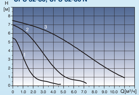
UPS 32-80, UPS 32-80 N
