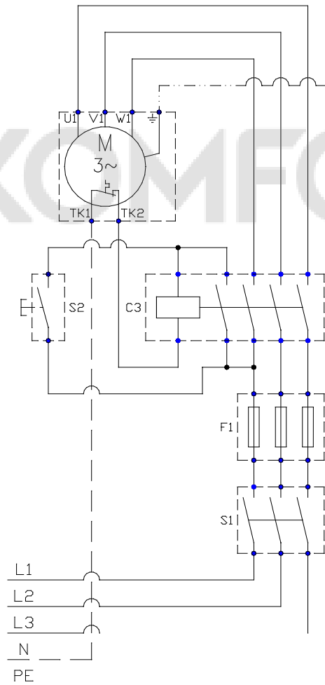
3-phase motor, bimetallic switch (TKO) thermal protection
