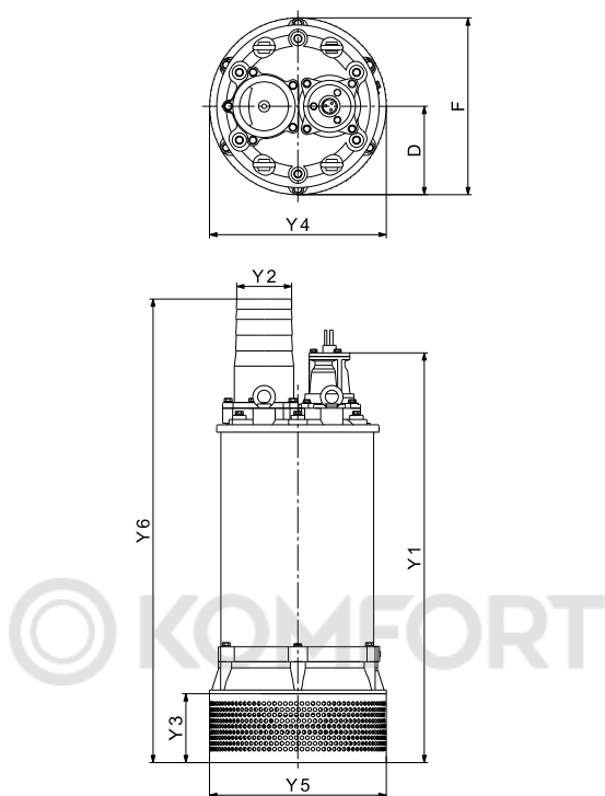
Fig. 3 Dimensions of pump with hose connection
