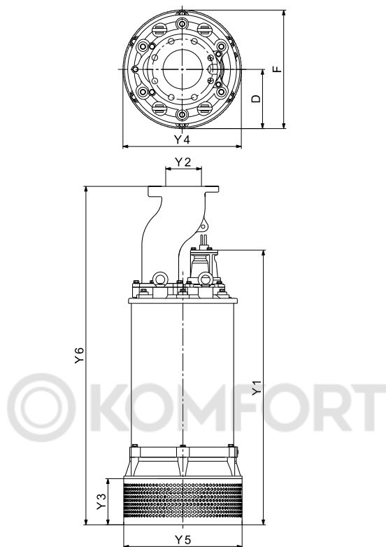
Fig. 4 Dimensions of pump with flange connection
